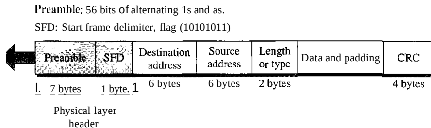
Figure 13.4 802.3 MAC frame
