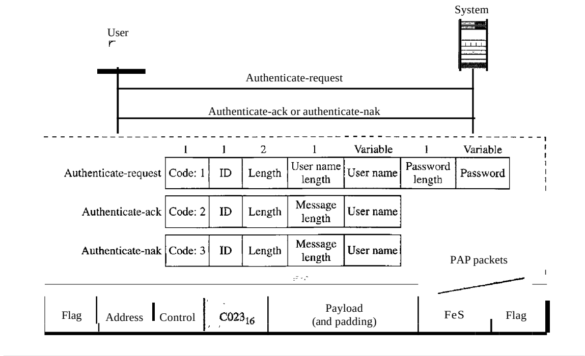
Figure 11.36 PAP packets encapsulated in a PPP frame
