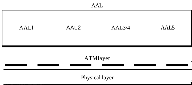
Figure 18.16 ATM layers
