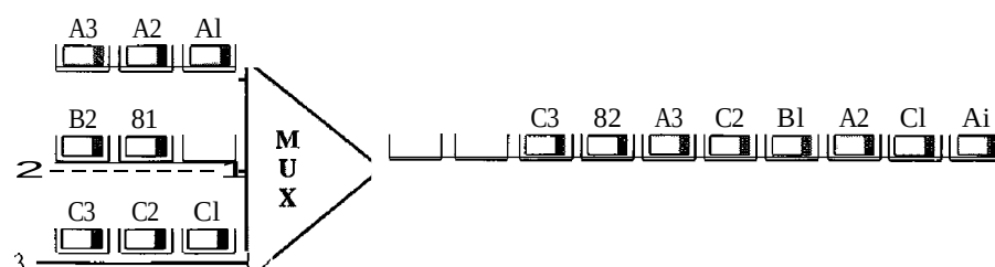
Figure 18.8 ATM multiplexing
