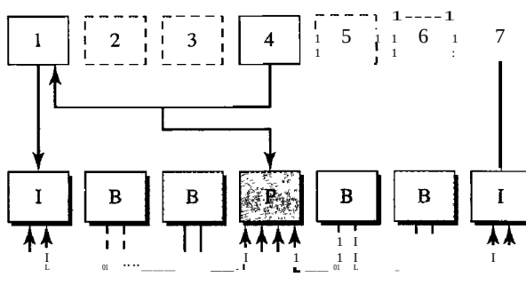
Figure 29.9 MPEG frame construction
