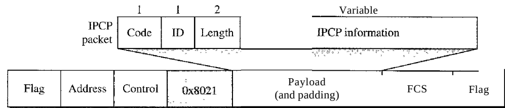
Figure 11.38 IPCP packet encapsulated in PPP frame
