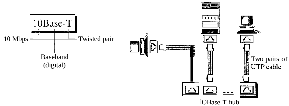
Figure 13.12 IOBase-T implementation
