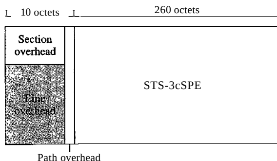
Figure 17.15 A concatenated STS-3c signal
