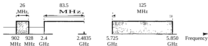
Figure 14.14 industrial, scientific, and medical (ISM) band
