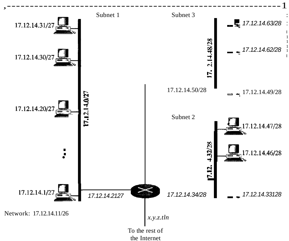
Figure 19.7 Configuration and addresses in a subnetted network
