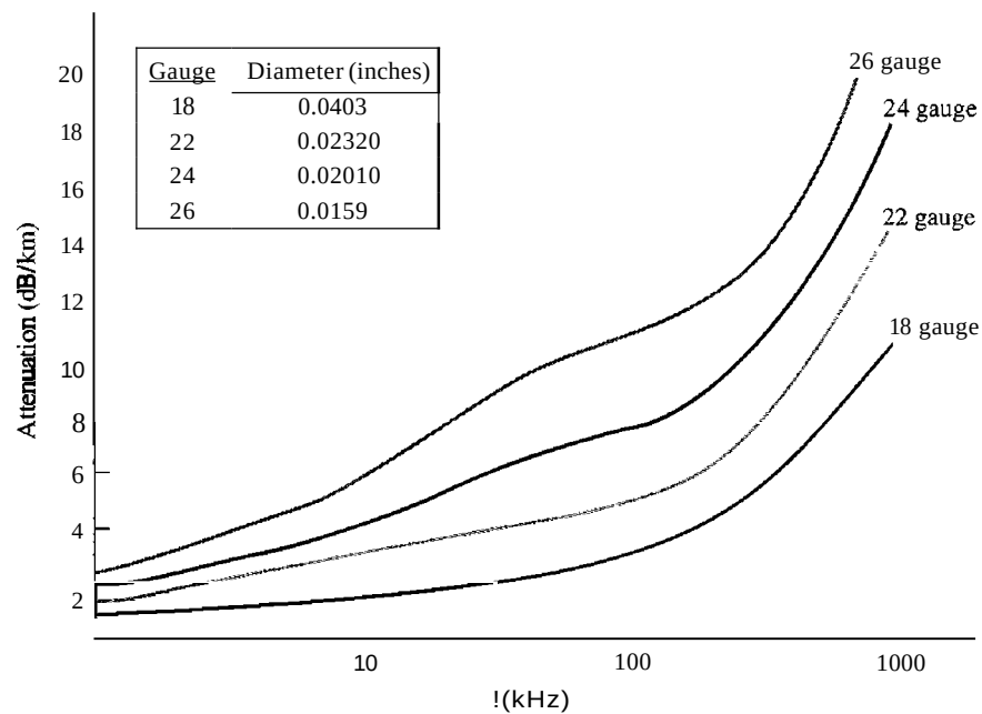
Figure 7.6 UTP performance
