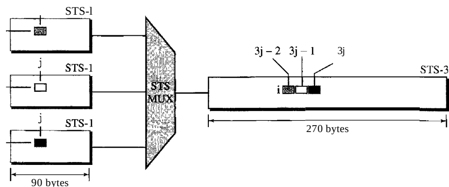
Figure 17.13 Byte interleaving
