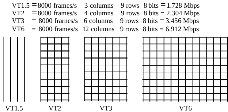
Figure 17.26 Virtual tributary types
