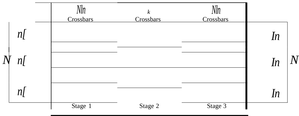
Figure 8.18 Multistage switch
