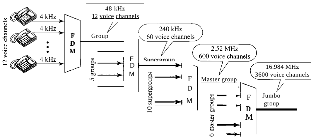
Figure 6.9 Analog hierarchy
