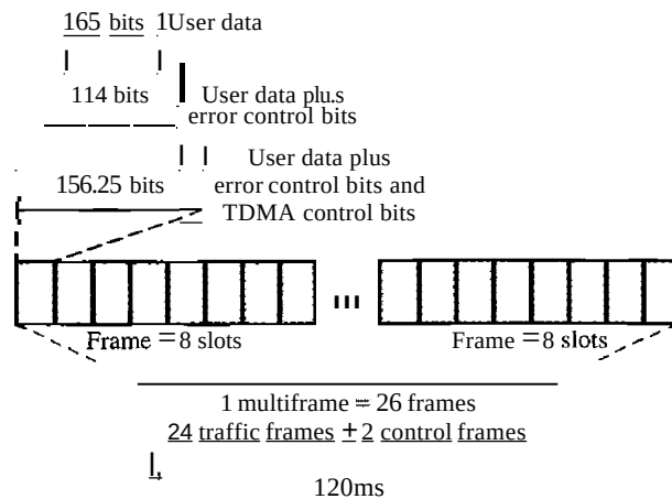
Figure 16.9 Multiframe components
