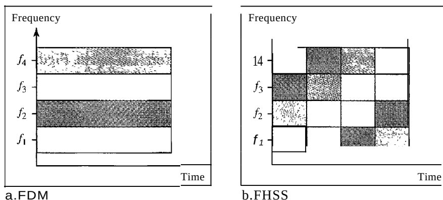
Figure 6.31 Bandwidth sharing
