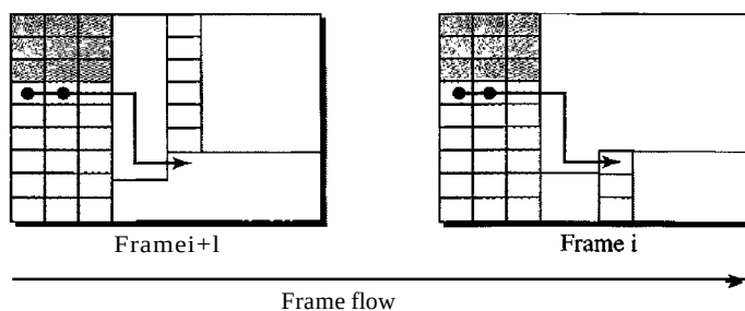
Figure 17.11 The use of HI and H2 pointers to show the start of an SPE in a frame
