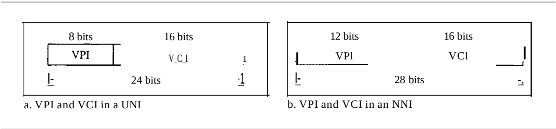
Figure 18.13 Virtual connection identifiers in UNIs and NNIs
