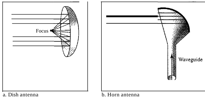
Figure 7.21 Unidirectional antennas
