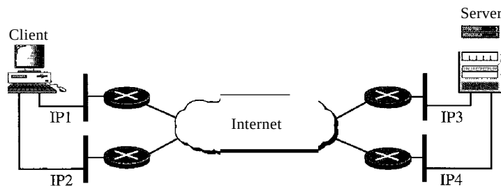
Figure 23.28 Multihoming concept
