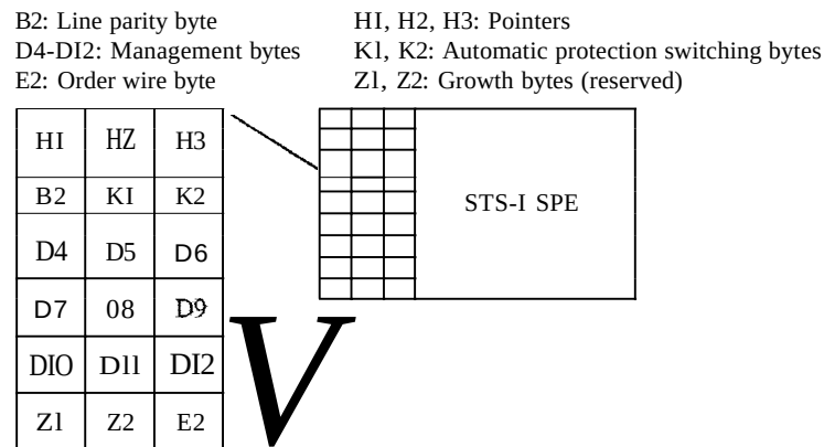
Figure 17.8 STS-I frame: line overhead
