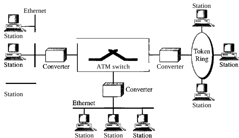
Figure 18.26 Legacy ATMLAN
