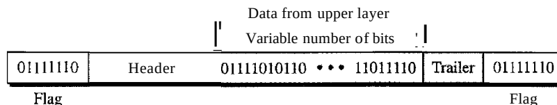
Figure 11.3 A frame in a bit-oriented protocol
