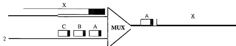
Figure 18.6 Multiplexing using different frame sizes
