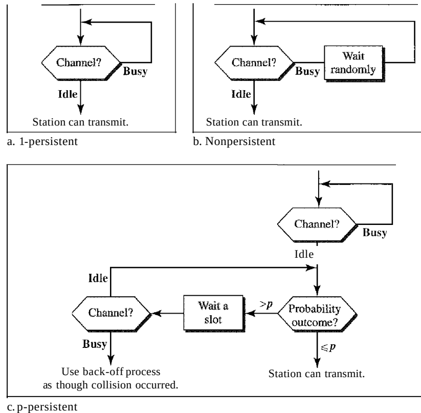
Figure 12.11 Flow diagram for three persistence methods
