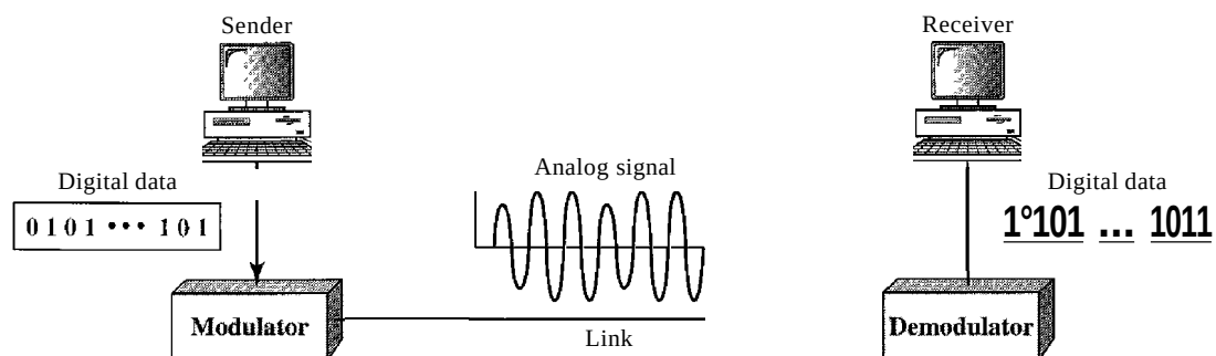
Figure 5.1 Digital-to-analog conversion
