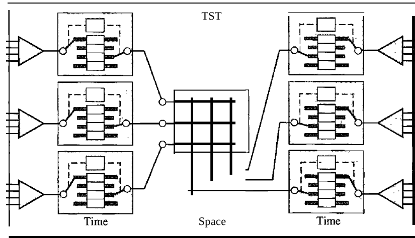
Figure 8.20 Time-space-time switch
