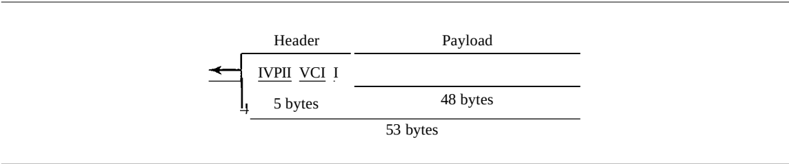
Figure 18.14 An ATM cell
