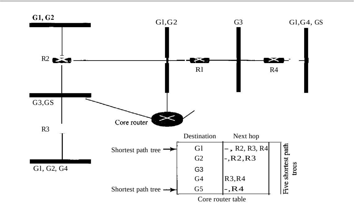
Figure 22.38 Group-shared tree approach
