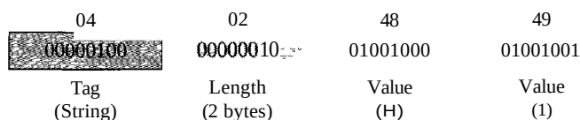
Figure 28.12 Example 28.2, OCTETSTRING "HI"
