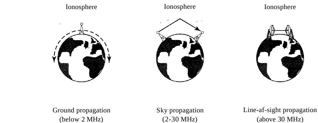
Figure 7.18 Propagation methods
