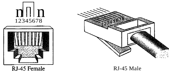
Figure 7.5 UTP connector
