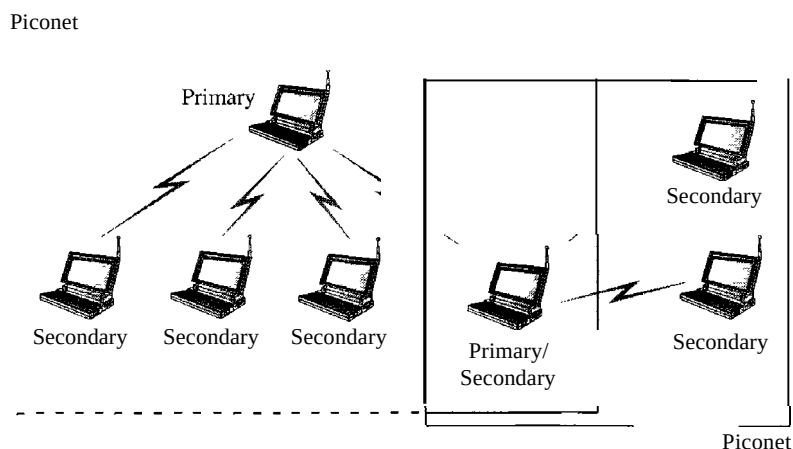
Figure 14.20 Scatternet
