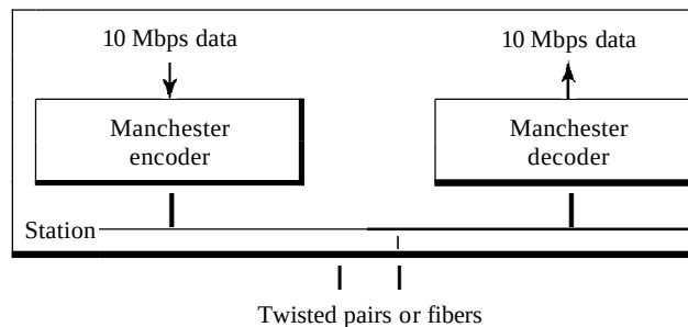
Figure 13.9 Encoding in a Standard Ethernet implementation
