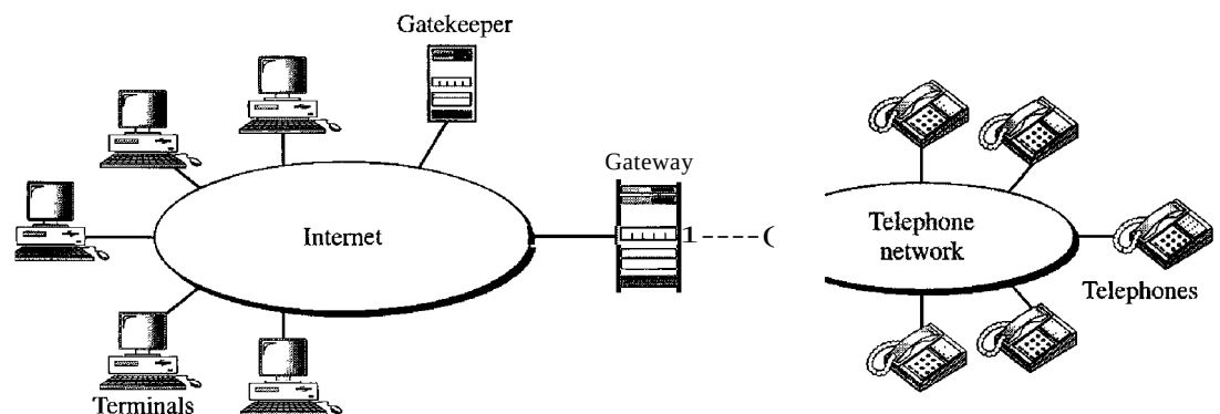
Figure 29.25 H.323 architecture
