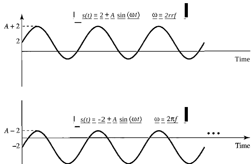
Figure C.3 Vertical shifting of sine waves
