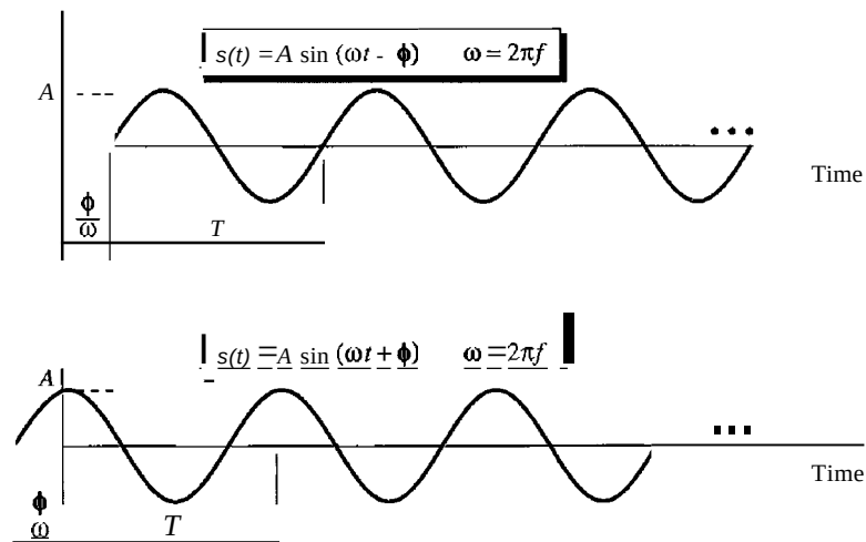
Figure C.2 Two horizontally shifted sine waves
