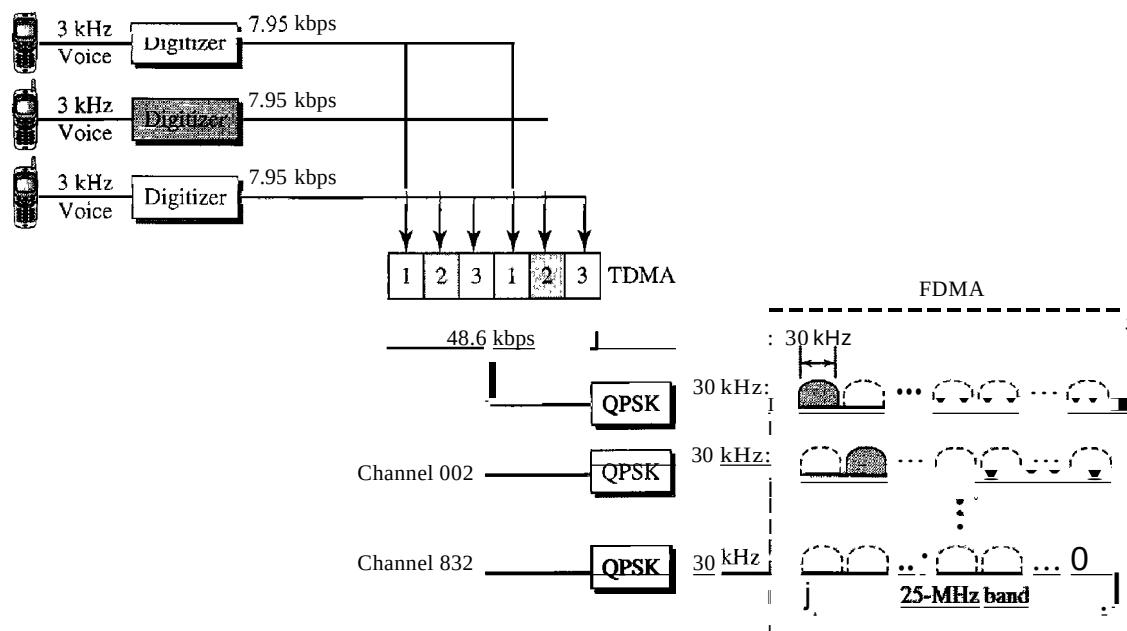
Figure 16.6 D-AMPS
