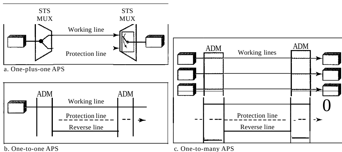
Figure 17.20 Automatic protection switching in linear networks
