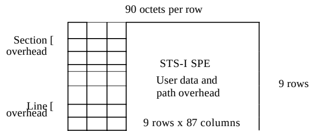
Figure 17.6 STS-1 frame overheads
