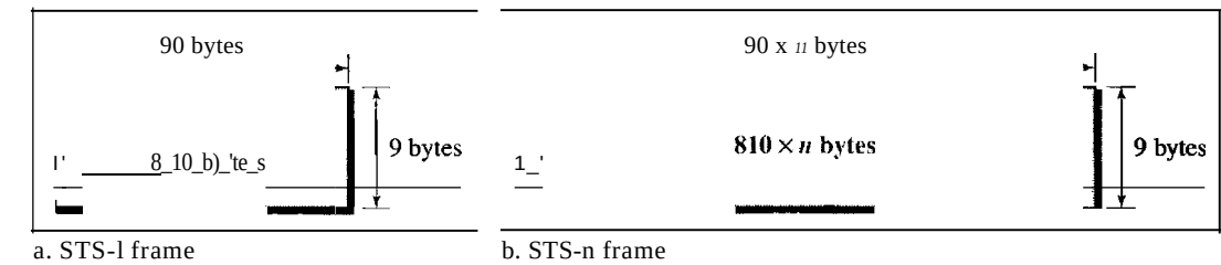
Figure 17.4 An STS-1 and an STS- n frame
