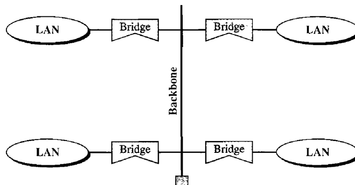
Figure 15.12 Bus backbone
